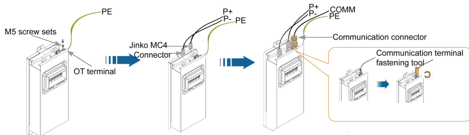
Connection Diagram
