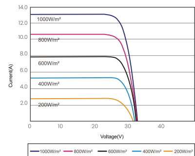
I-V CURVES OF PV MODULE(410W)
